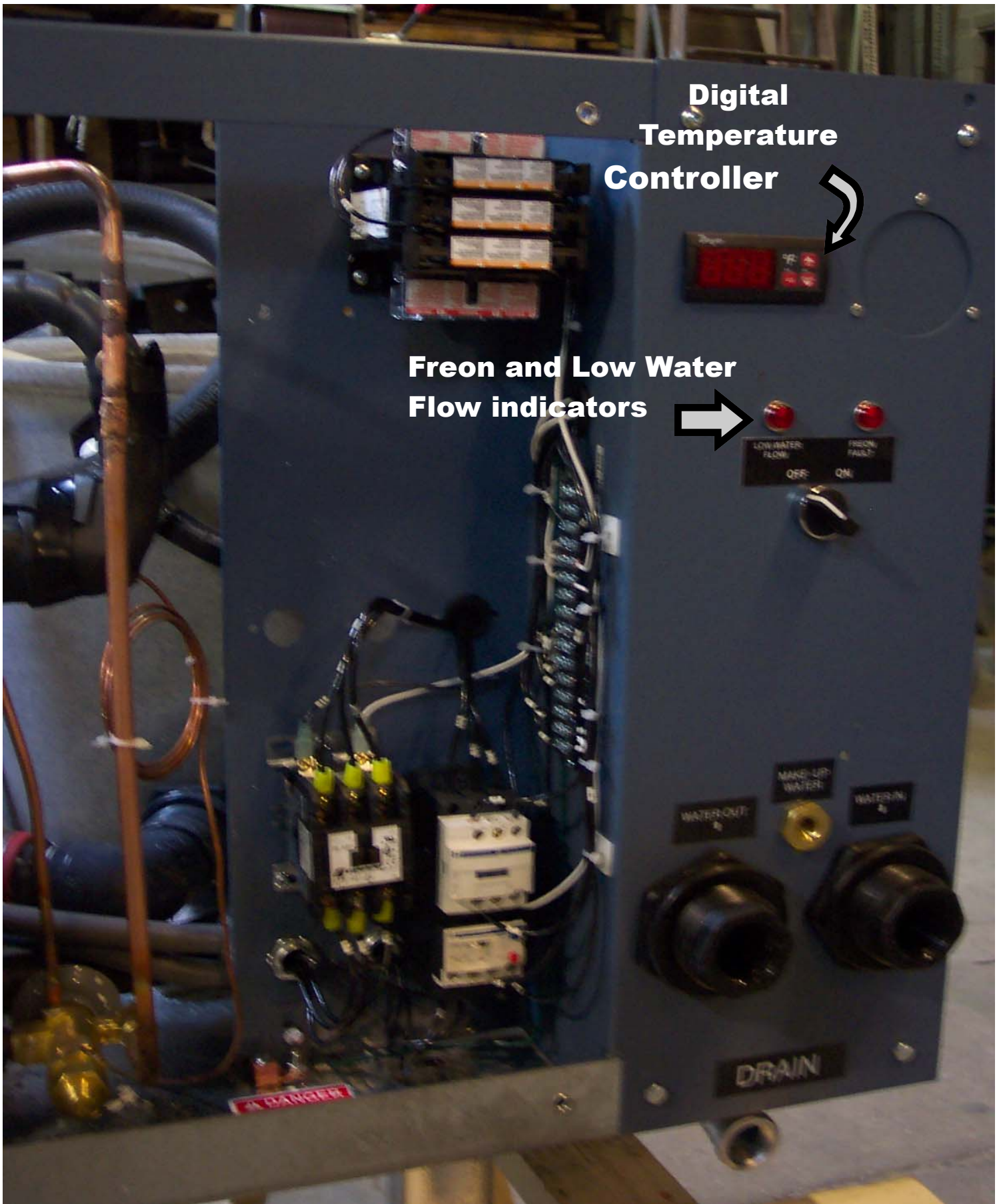
FEATURES FOUND IN ALL UNITROL CHILLERS
